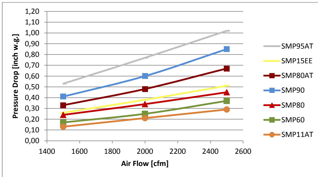
Fig. 1: Pressure Drop Data of Aeolus 4 inch Mini Pleat Panel Filters 24x24x4", Recommended airflow: 2000 cfm / 500 fpm; Independently Tested
